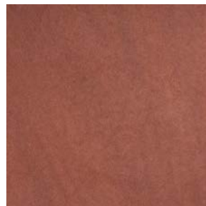
RED SANDSTONE
