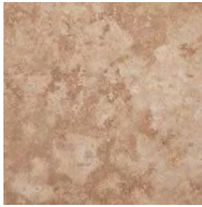
HARAST LIMESTONE
